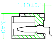
SECTION E-E
